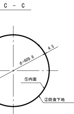
C 2-PL 300x4. 5x964 (SS400)
