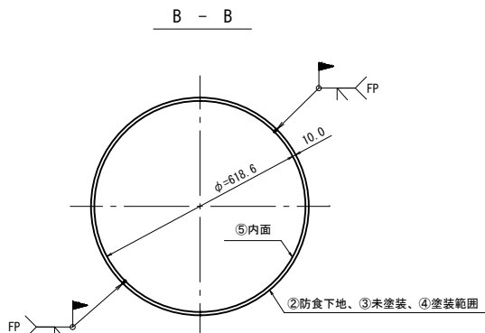
B 2-PL 300x10x980 (SM400A)
